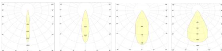
15° Reflector
