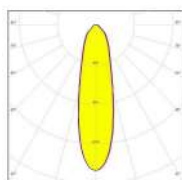
30° Lens
