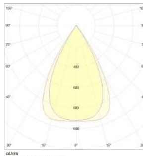
50° Light Beam
