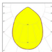
90° Lens
