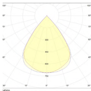
80° Light Beam
