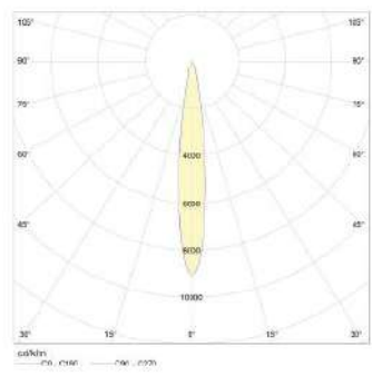
15° Reflector
