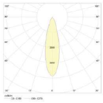
30° Reflector
