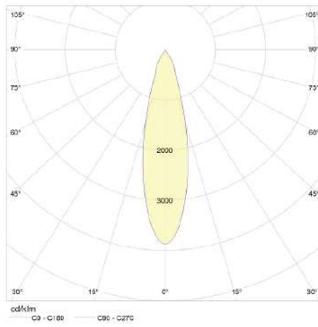
30° Reflector
