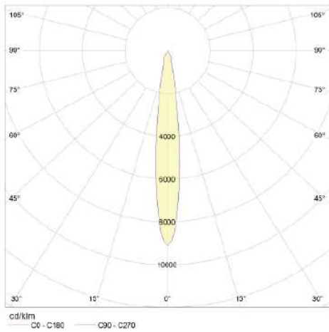
15° Reflector
