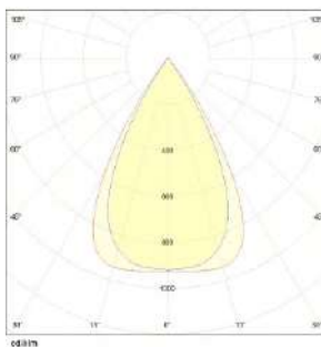
50° Light Beam
