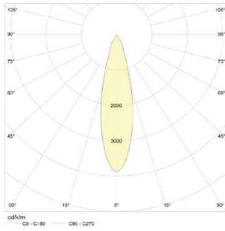
30° Reflector
