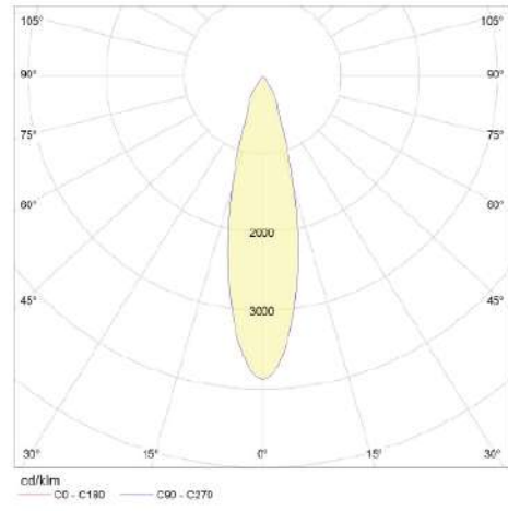
30° Reflector
