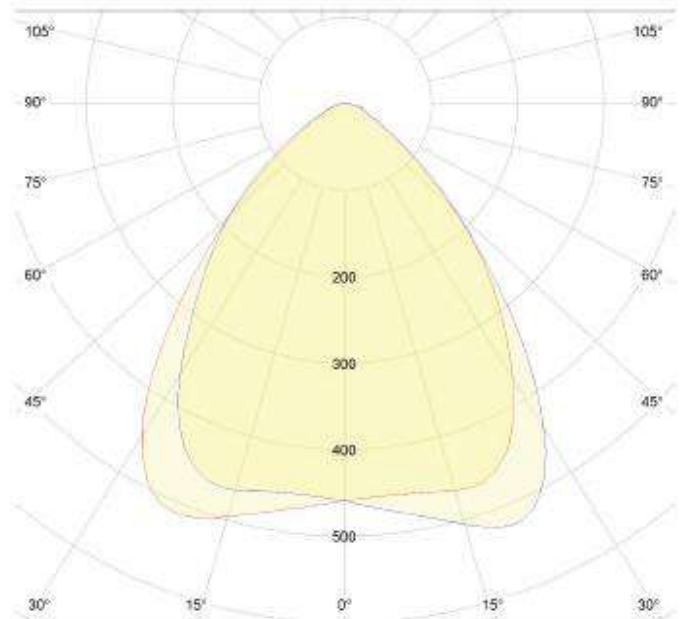
98° Lens
