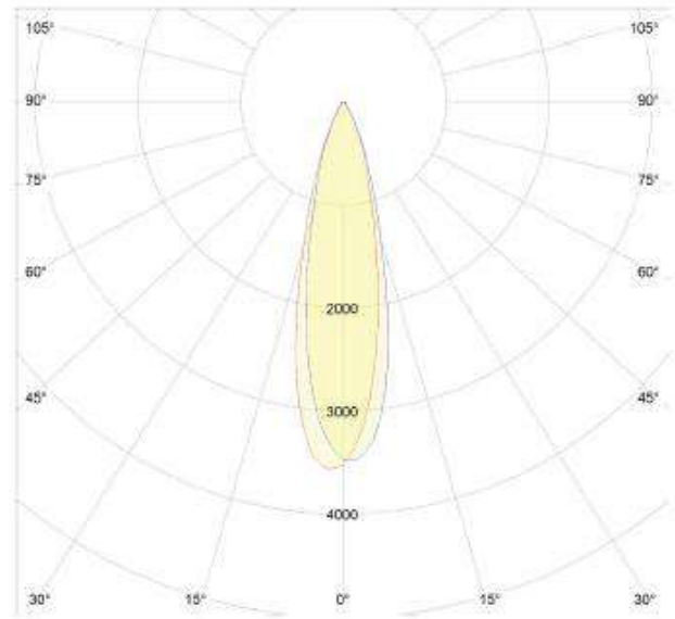
25° Lens
