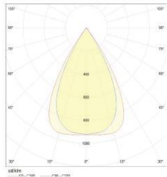
50° Light Beam
