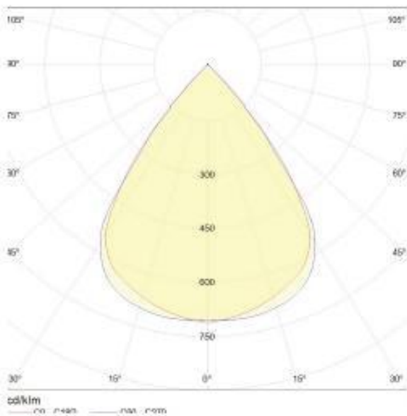
80° Light Beam
