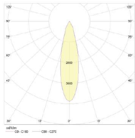
30° Reflector
