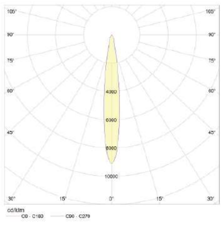
15° Reflector
