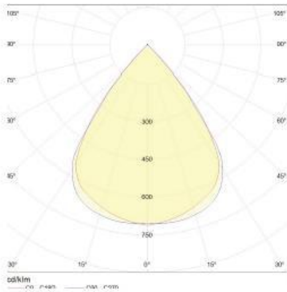
80° Light Beam
