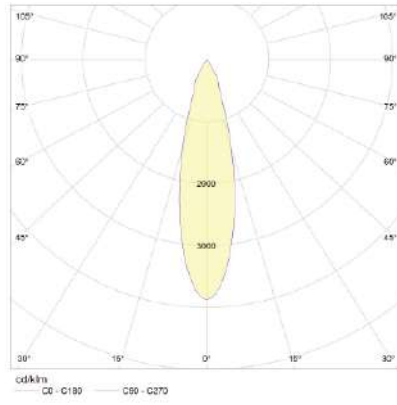
30° Reflector
