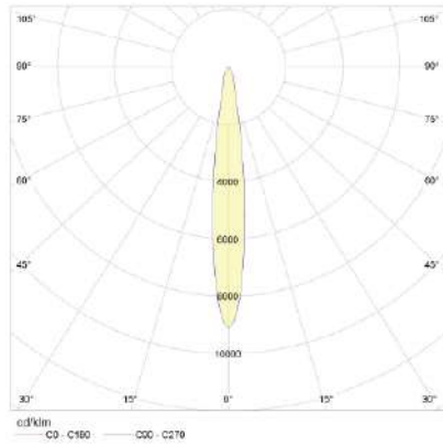
15° Reflector
